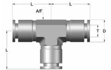
GXUT "T" Tubo-Tubo-Tubo
